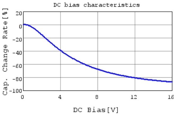
GRM188B31C225KE14 C-DC bias capchange, 20.0c
