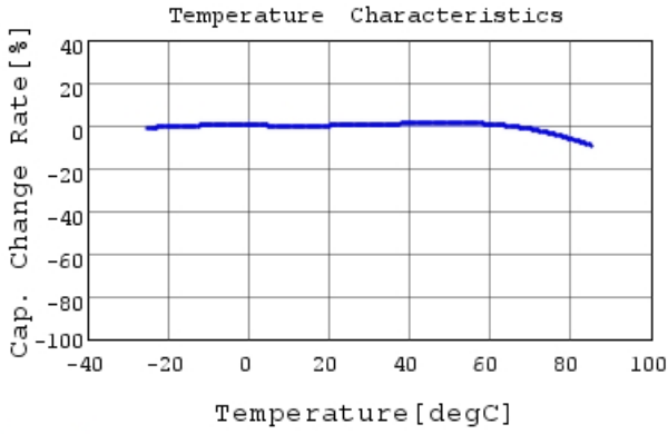
GRM188B31C225KE14 C-Temp. capchange, DC0.0V,
