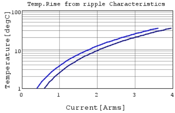
GRM188B31C225KE14 Temp.rise — 500kHz
