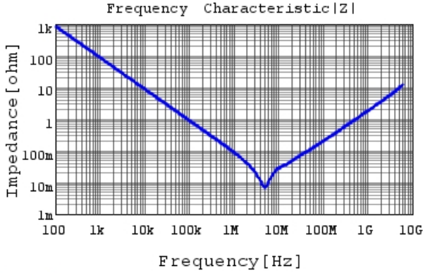
GRM188B31C225KE14 |Z| DCOV, 20degC
