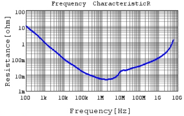
GRM188B31C225KE14 R DCOV, 20degC
