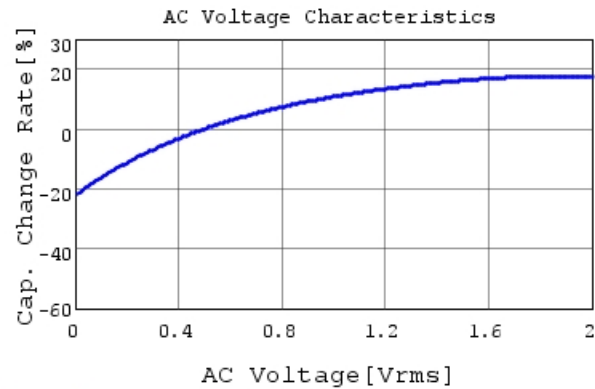
GRM188B31C225KE14 C-AC Voltage capchange, Dc
